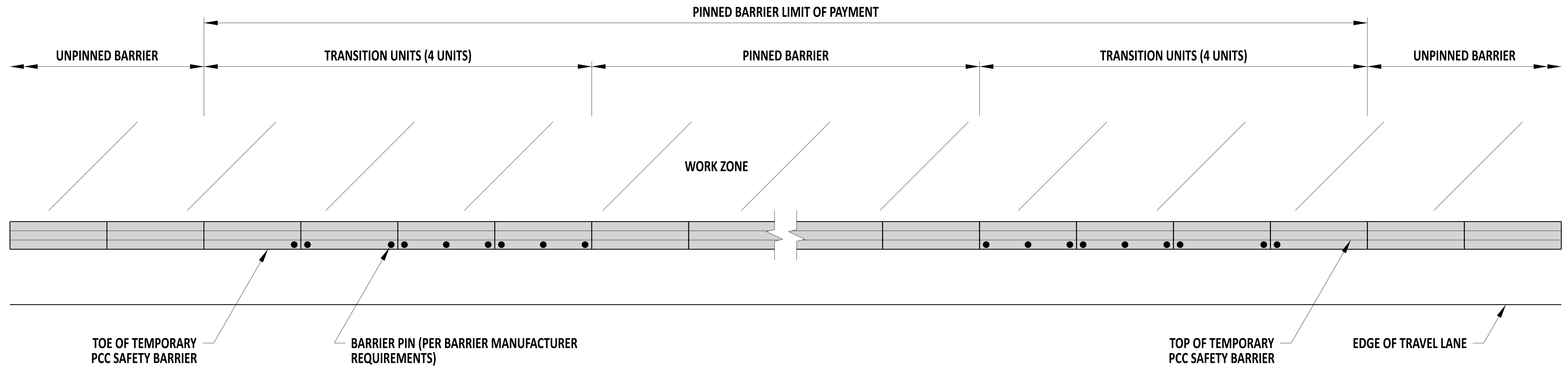
PLAN VIEW
