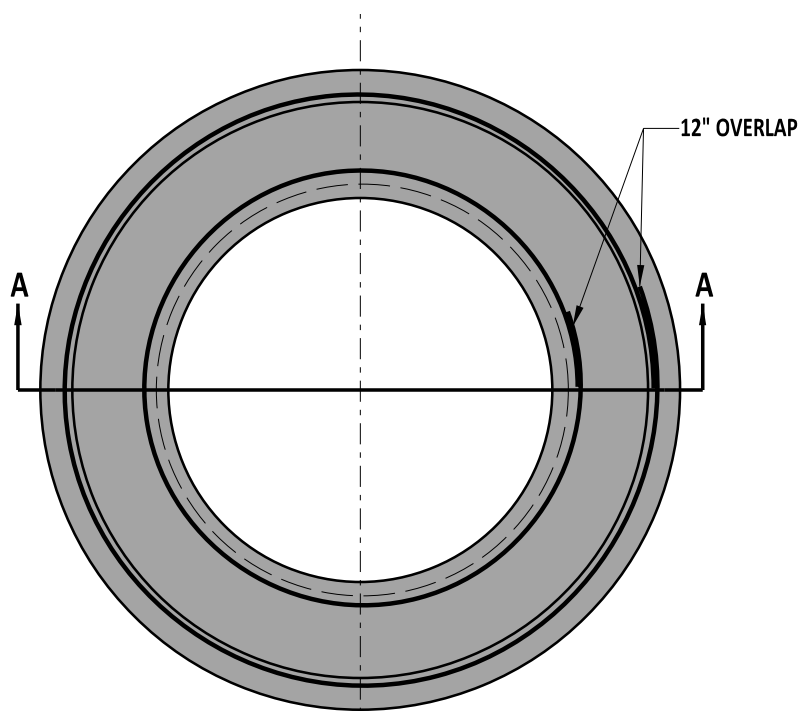
GRADE RING
