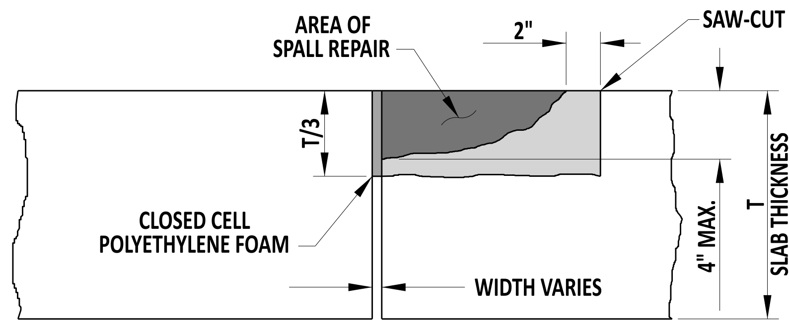
SECTION WITH SPALL ADJACENT TO JOINT
