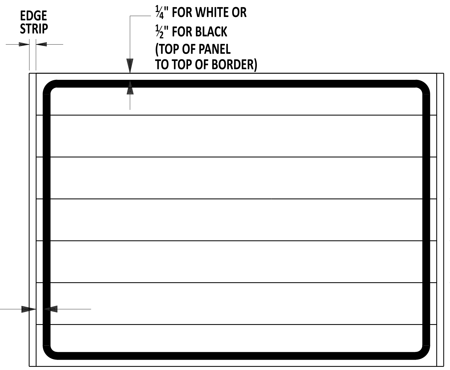
BORDER DETAIL
