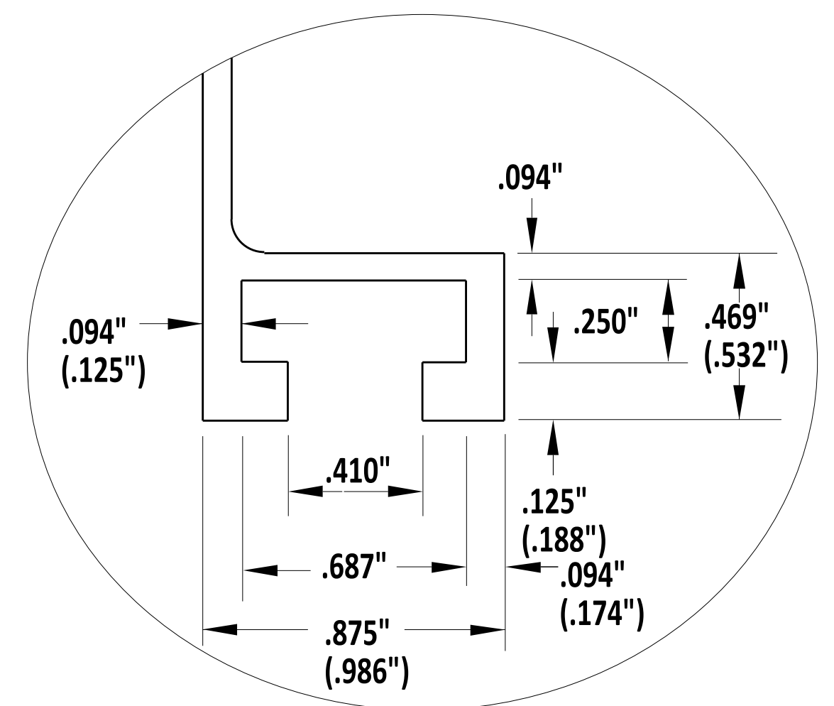
DETAIL A
